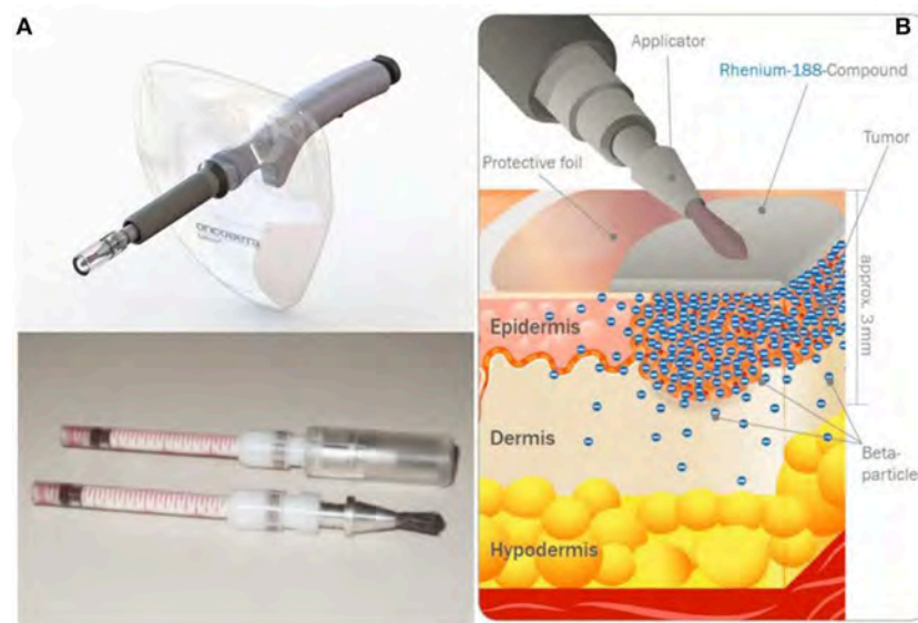
FIGURE 10 | Rhenium-SCT device developed by OncoBeta ® GmbH (Garching, Germany). Applicator and dispensing carpoules filled with 188 Re-cream (A) and illustration of the principle (B) (Courtesy of Dr. Shannon Brown III, OncoBeta ® ).
